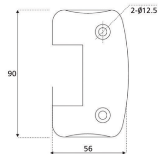
DSH-33 Glass to Glass 135° Hinge
