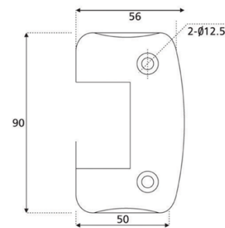
DSH-22 Glass to Glass 180° Hinge
