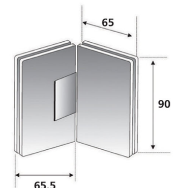
DSH-3 Glass to Glass 135° Hinge
