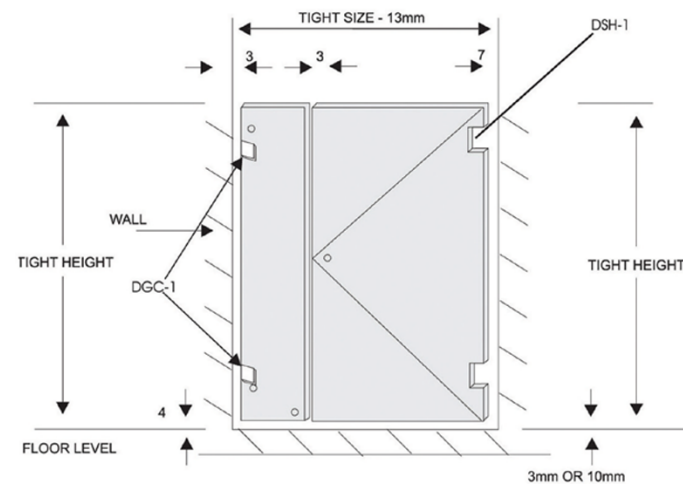
WALL / GLASS LAYOUT
