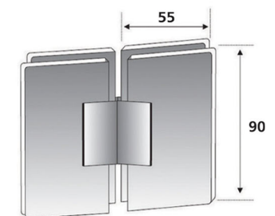
DSH-2 Glass to Glass 180° Hinge
