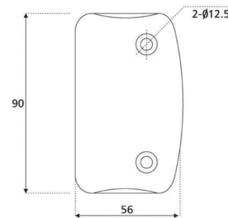
DSH-11 Wall to Glass Hinge
