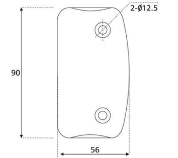
DSH-55 Wall to Glass Fixed Hinge
