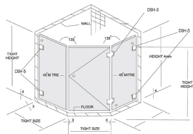
135 WALL / GLASS LAYOUT
