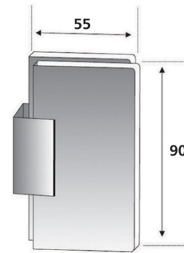
DSH-5 Wall to Glass Fixed Hinge
