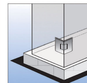
DSH-4 Glass to Glass 90° Hinge
