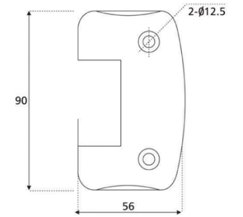
DSH-44 Glass to Glass 90° Hinge
