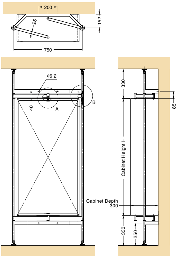
RB-600-CH Floor-to-ceiling type
