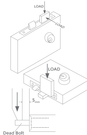
Lever handle locks SXEVE/MVSX
